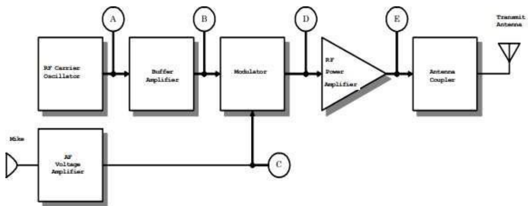
Fig.1. Low-Level AM Transmitter Block Diagram
