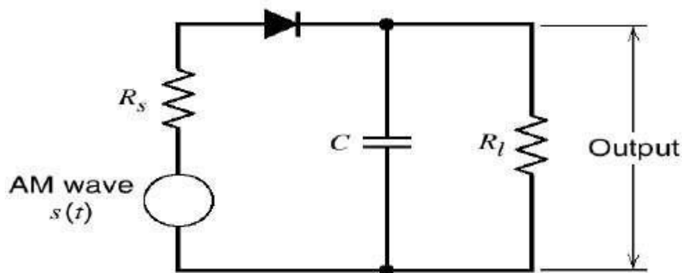
Envelope Detector
