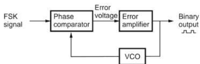
Fig. FSK detection using PLL
